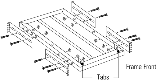
Figure 6. Frame Assembly
