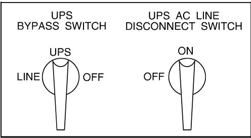
Figure 31. Make-Before-Break Bypass Switch
