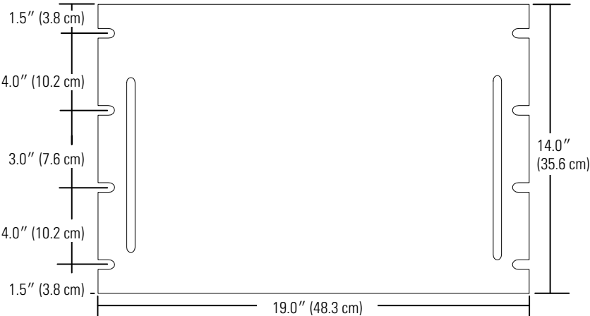
Figure 7. RBC-1 and RBC-2 Front Panel Bolt Slot Measurements
