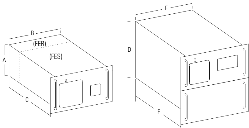
Figure 1. UPS Dimensions
